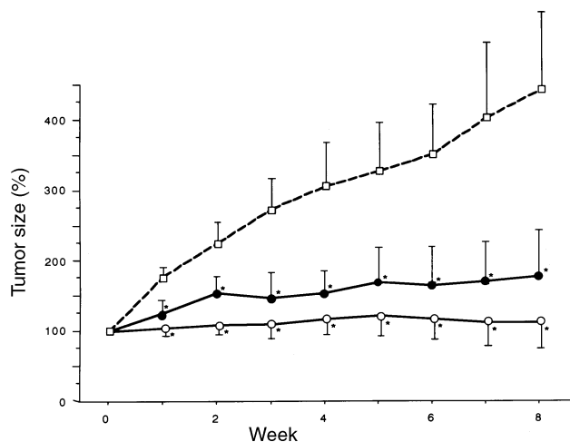
Fig. 2. Weekly changes in tumor size expressed as a percentage of the size measured on day 0 (mean \pm SD). \square , I-A; \bullet , I-B; \circ , I-C. n=11 in each group. Groups I-B and I-C were significantly different from the control group ( P<0.05 ) throughout the 8-week period.
